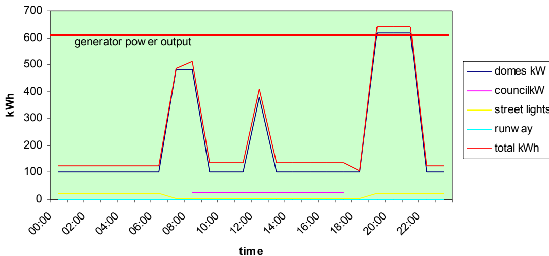
Figure 9 Total energy used in Codrington over 24 hrs
