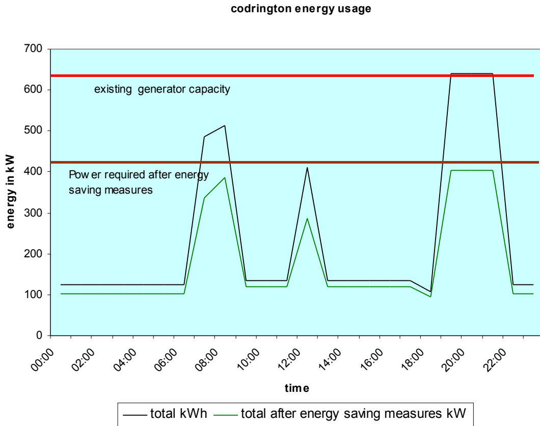
Figure 12 Energy requirement of Codrington with energy saving measures in place.
