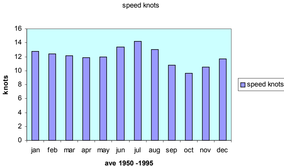
Figure 16 Average monthly wind speeds over 45 years (CWS, 2002)
