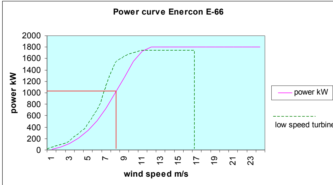
Figure 20 Power curve of typical European 1800kW wind turbine with low speed turbine approximation in green.
