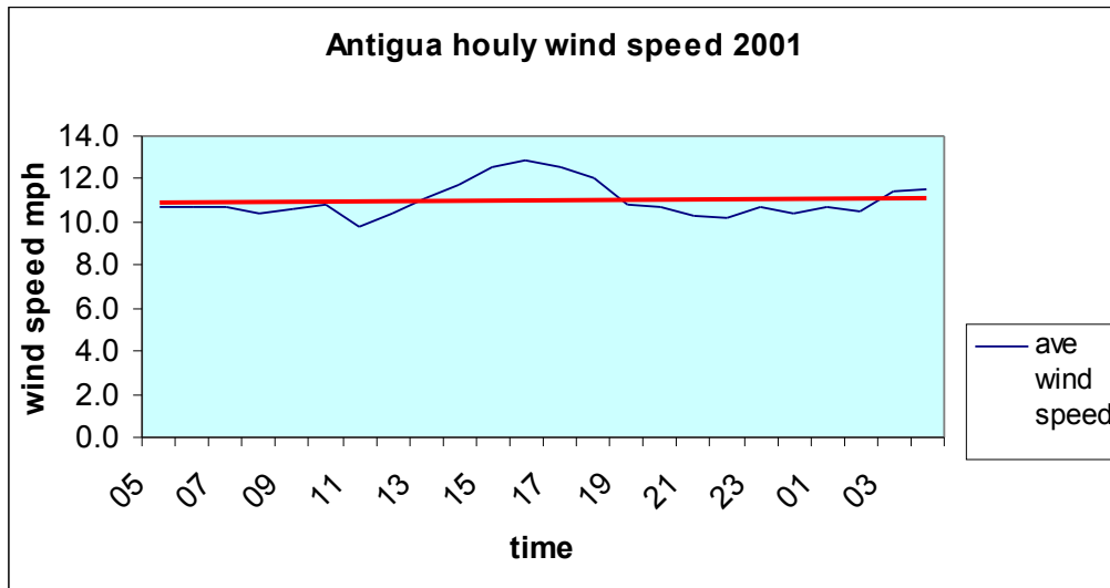
Figure 18 Annual mean hourly wind speed for 2001. (Data provided by AMS, 2002)
